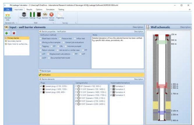
Software graphical user interface for defining well barrier elements and related properties.
