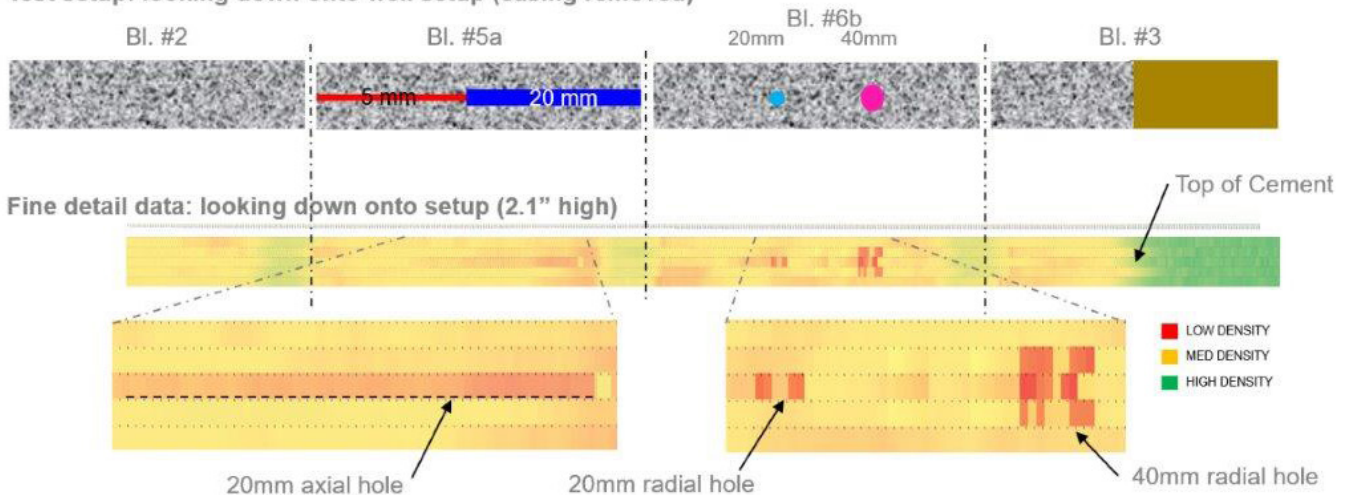
2-D image showing cement defects detected by X-rays scanning four test blocks during the Visuray VR360 concept experiment.
