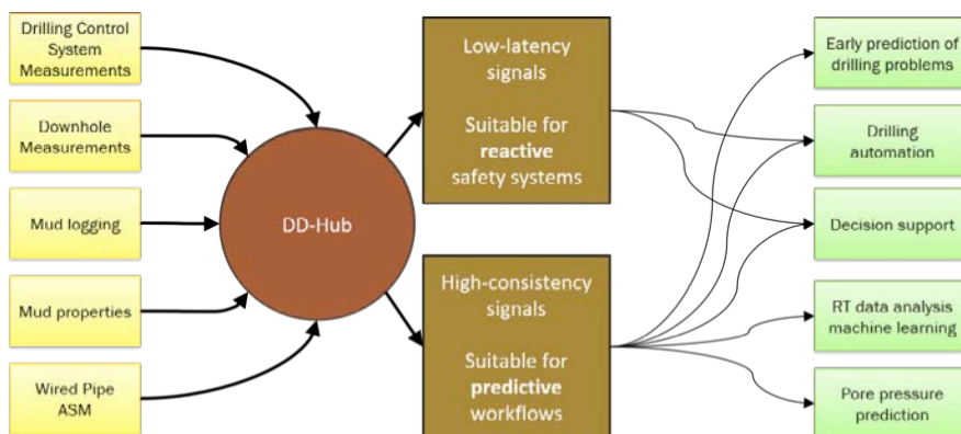
Flow of information during drilling – Intermediate interface reference implementation.
