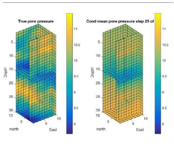
New methods for uncertainty prediction around a planned well path have been tested. From Paglia & Eidsvik (2017).
