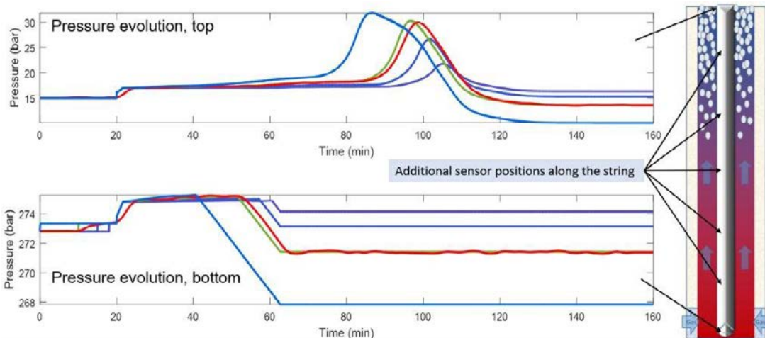
Gas kick event: Pressure recordings (red) and simulations (blue, best fit in green) with different kick volumes.
